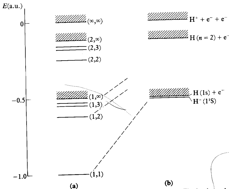
6.6 (a) The energy spectrum given by expression [6.32] with Z = 1 . The levels are labelled by (n_1, n_2) . (b) The energy spectrum of \text{H}^- .
